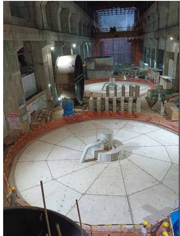
BOXING UP OF UNIT#1 & UNIT#2 (250 MW EACH) COMPLETED – 2000 MW SUBANSIRI LOWER (ARUNACHAL PRADESH)
